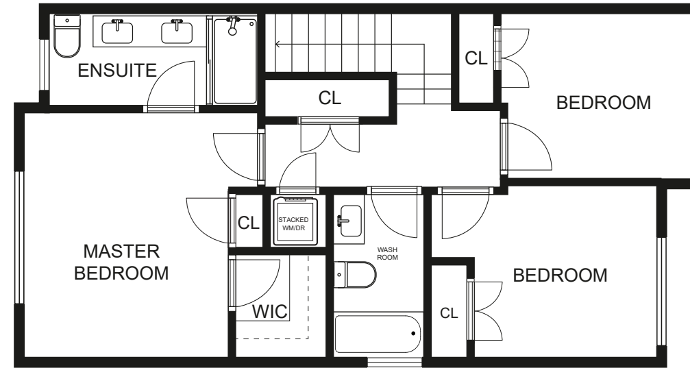
TOP FLOOR
