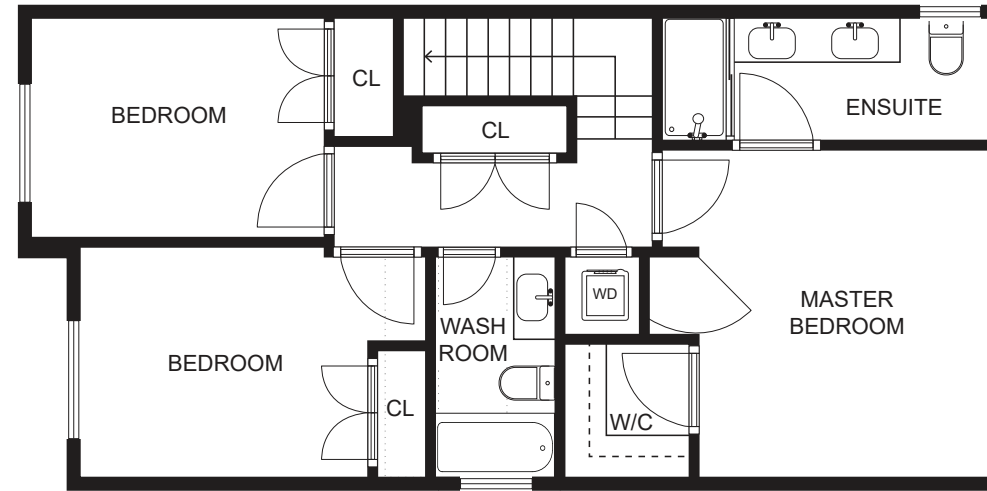
TOP FLOOR
